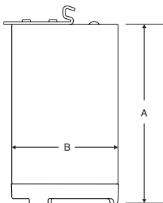
Fig. 26-1. Bucket Dimensions.
